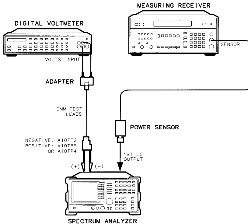
Figure 2-33. First LO Distribution Amplifier Adjustment Setup
