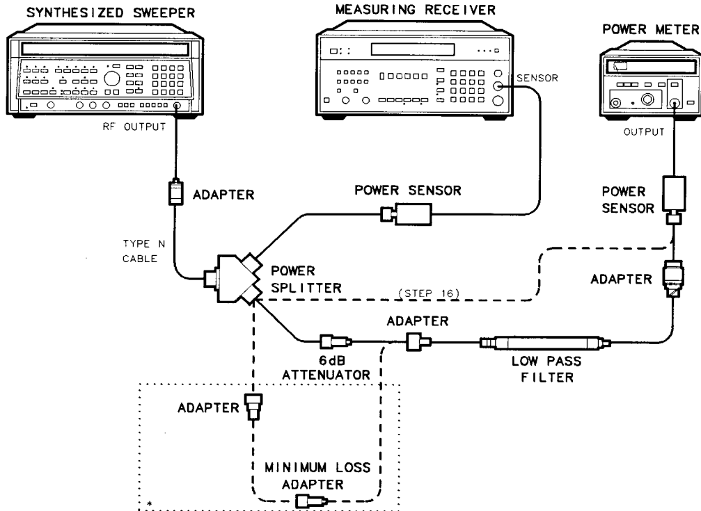
Figure 2-23. LPF Characterization
