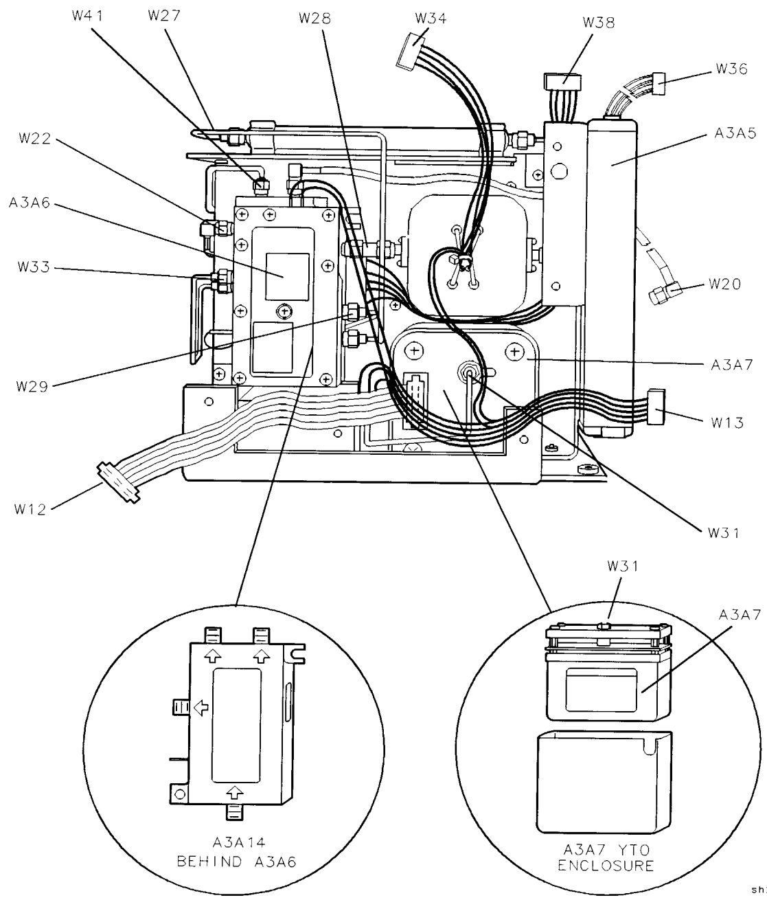
Figure 11-29. A3 Front-End Assembly, Right-Side View HP 8595E and HP 8596E (Options 009 and 010)
