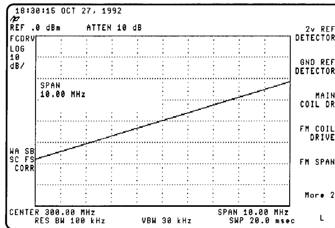
Figure 4-10. FM Coil Driver with \leq 10 MHz Span
