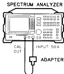
Figure 2-14. CAL AMPTD Adjustment Routine Setup
