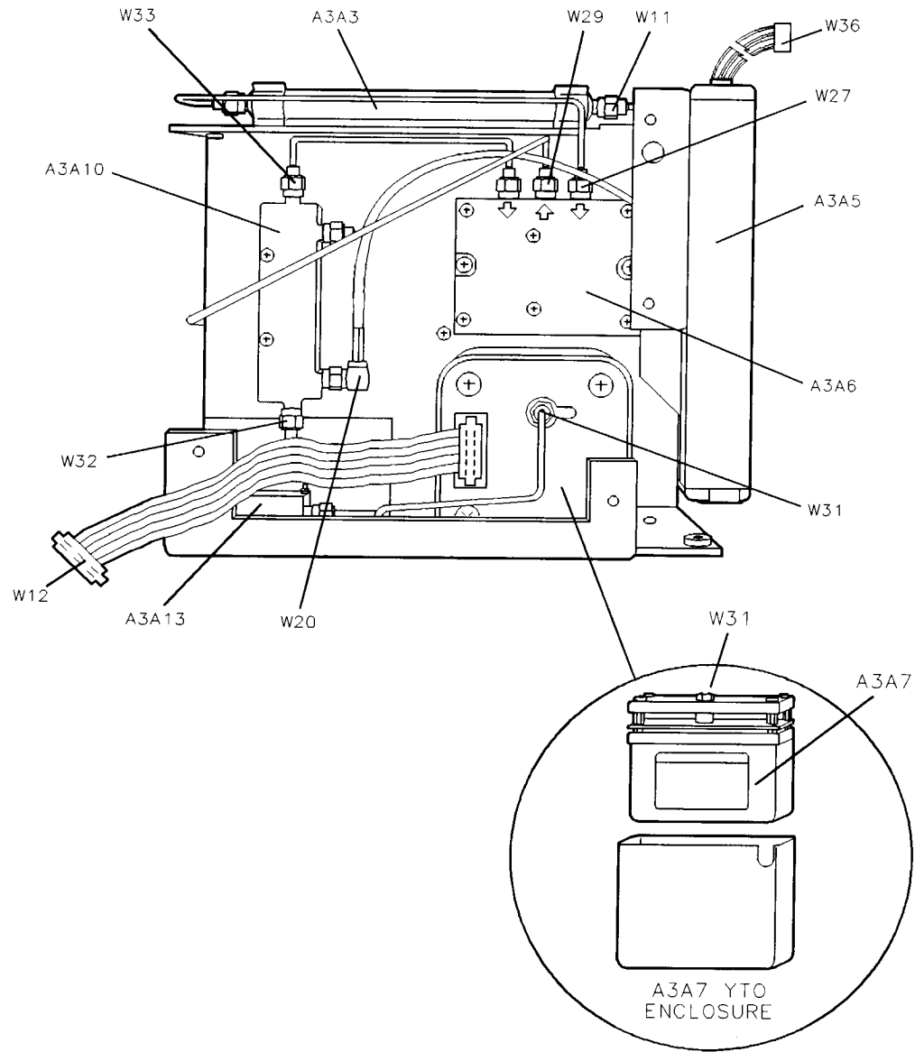
Figure 11-22. A3 Front-End Assembly, Right-Side View HP 8594E and HP 8594L
