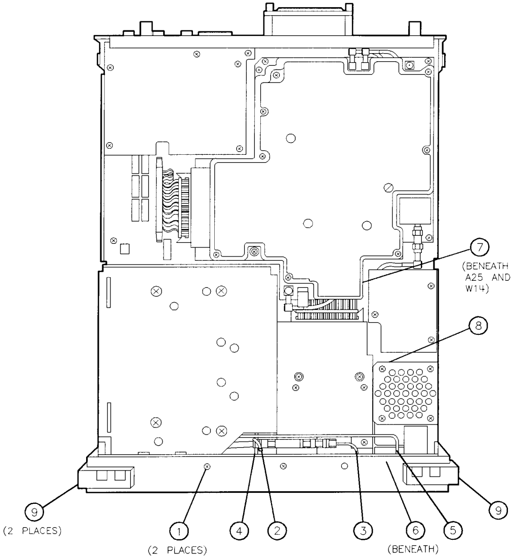
Figure 7-1. A1 Front-Frame Replacement
