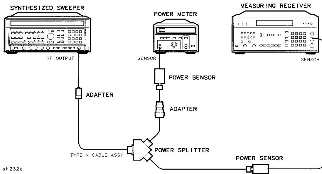
Figure 2-27. System Characterization Test Setup for 75 \Omega inputs
