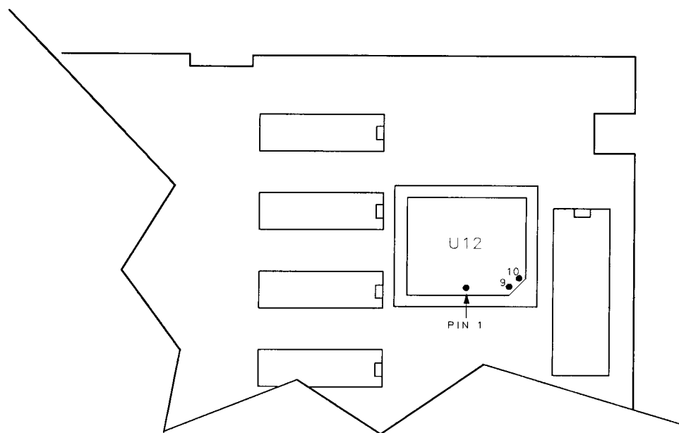
Figure 4-16. A16U12 Pin Location
