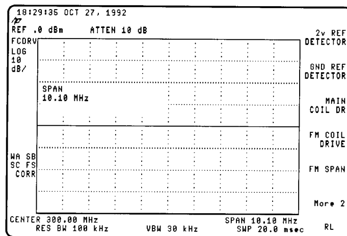
Figure 4-11. FM Coil Driver with >10 MHz Span
