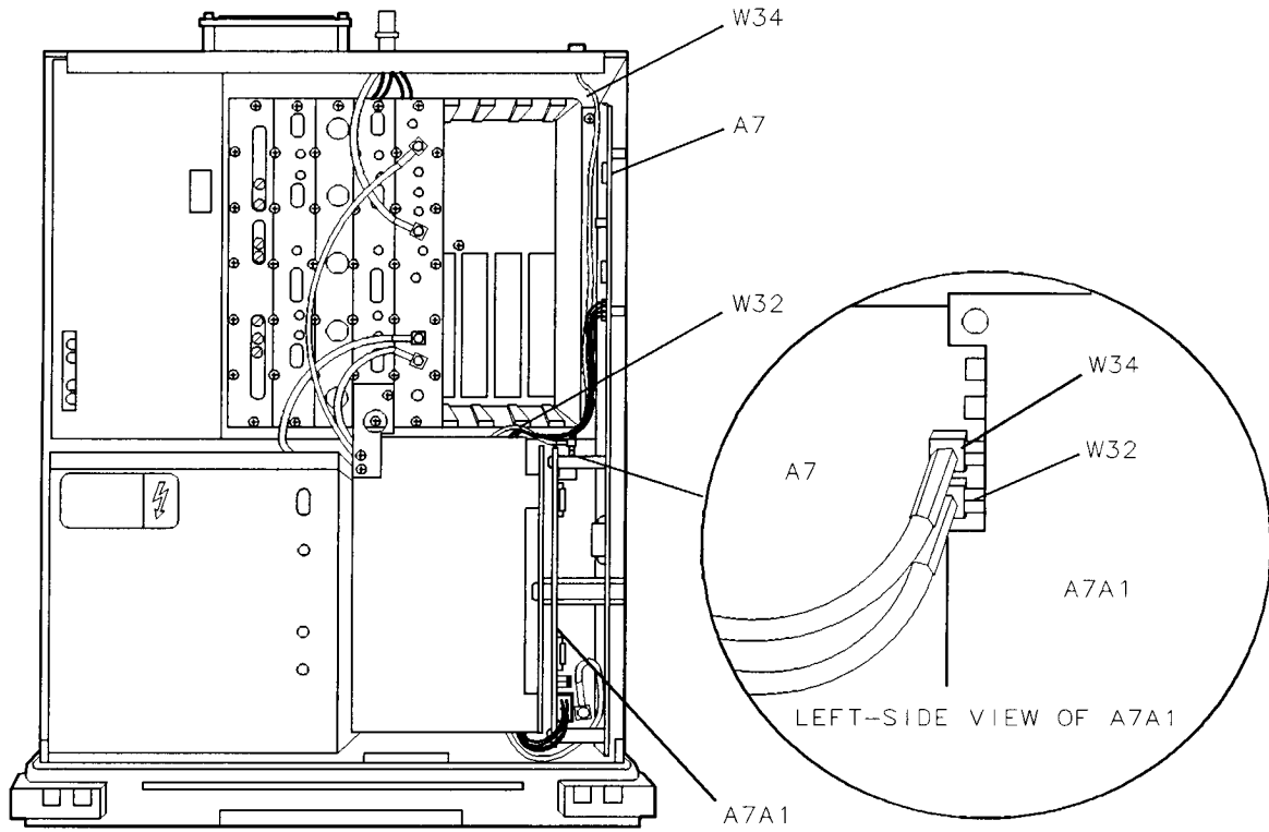
Figure 11-4. A7A1 Left-Side View HP 8590L, HP 8591C, and HP 8591E
