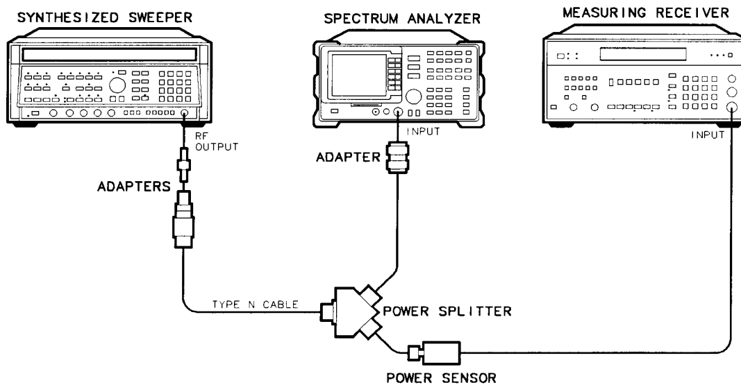
Figure 2-38. Absolute Amplitude Accuracy Verification
