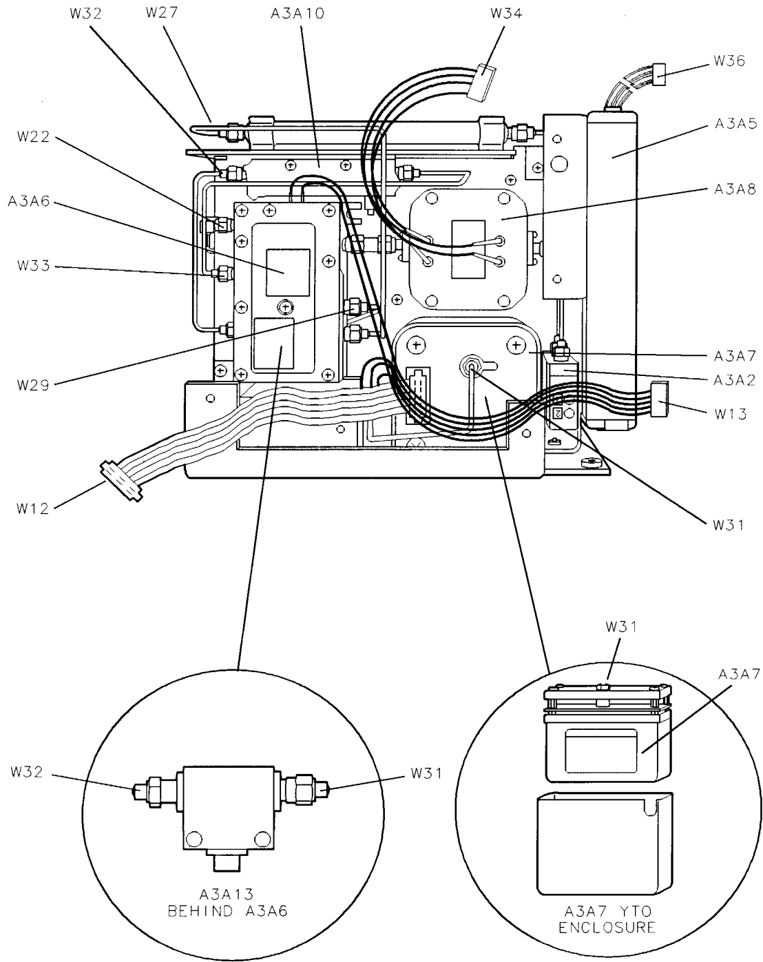
Figure 11-21. A3 Front-End Assembly, Right-Side View HP 8593E
