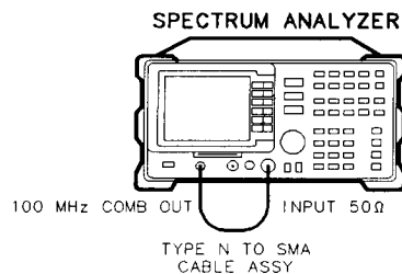
Figure 2-15. CAL YTF Adjustment Setup
