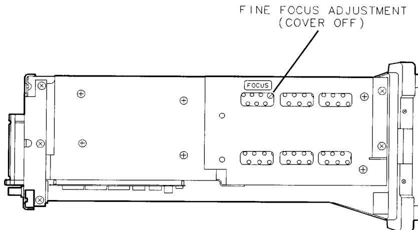
Figure 2-3. Focus Adjustment Location
