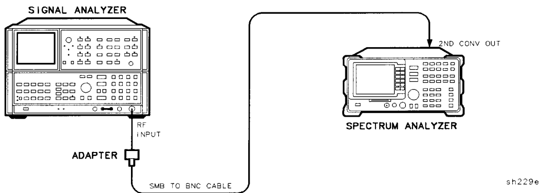
Figure 2-20. Second Mixer Match Adjustment Setup
