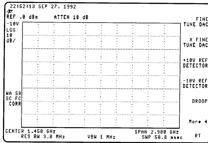
Figure 4-14. -10 V Reference Detector
