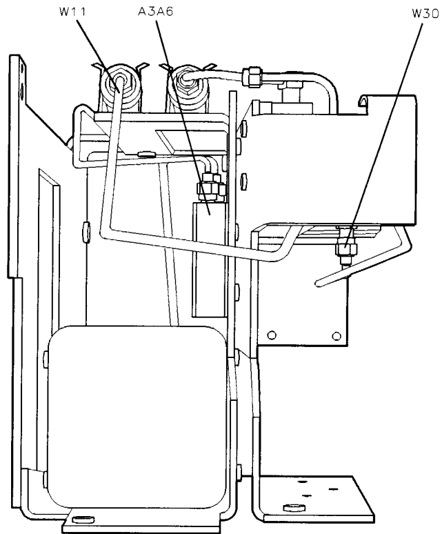
Figure 11-25. A3 Front-End Assembly, Rear View with A3A5 Removed HP 8594E (Options 009 and 010)
