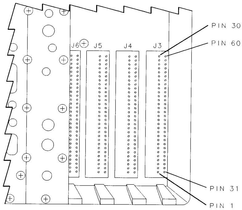
Figure 5-4. Card-Cage Connector Pin Designation
