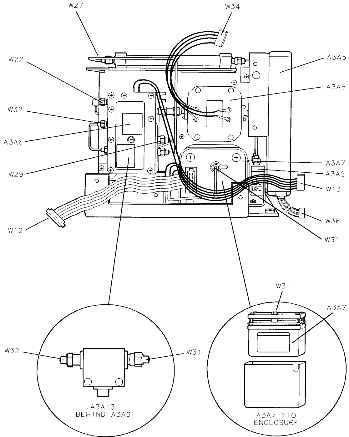
Figure 11-20. A3 Front-End Assembly, Right-Side View HP 8592L
