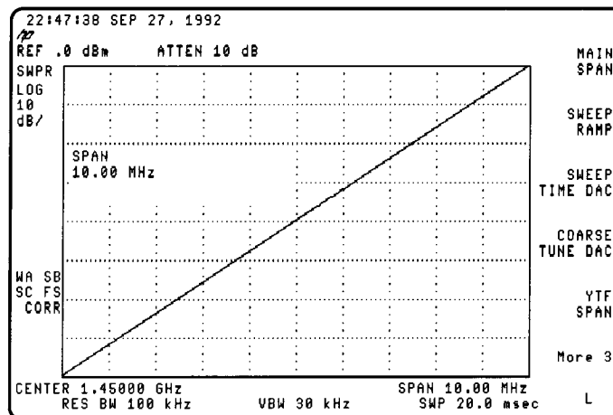
Figure 4-12. Typical Sweep Ramp Display
