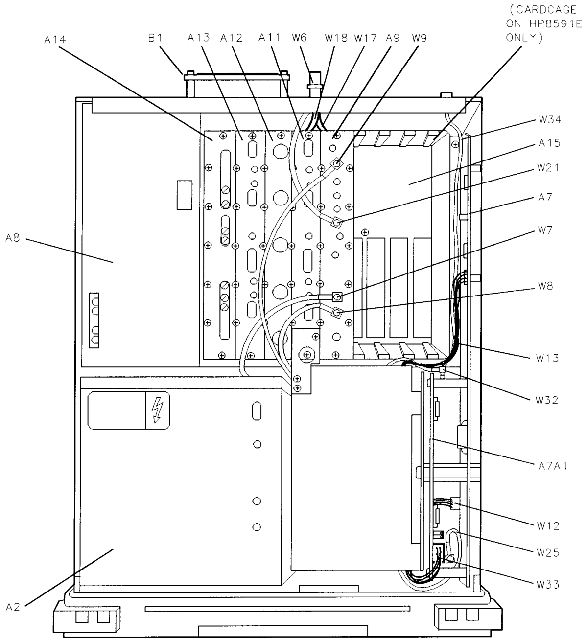
Figure 11-2. Instrument Top View HP 8590L, HP 8591C, and HP 8591E
