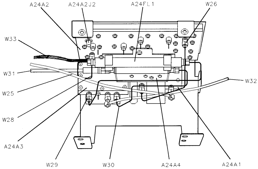
Figure 11-18. A24 Tracking Generator HP 8591C (Option 011) and HP 8591E (Options 010 and 011)
