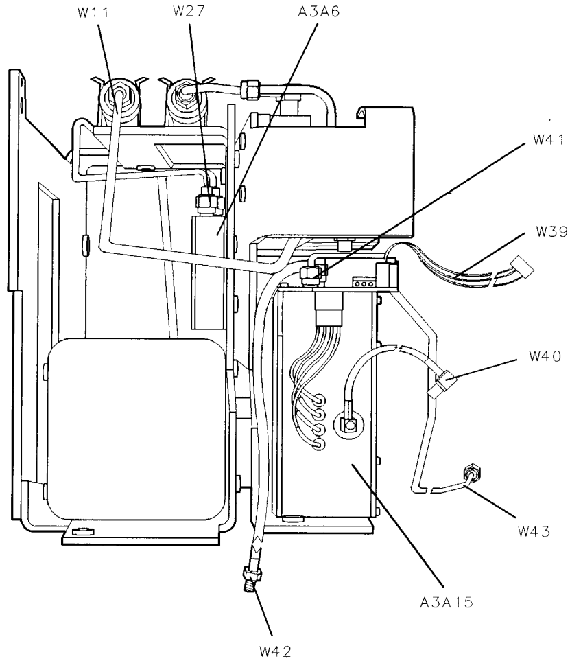
Figure 11-31. A3 Front-End Assembly, Rear View with A3A5 Removed HP 8594E (Options 009 and 010)
