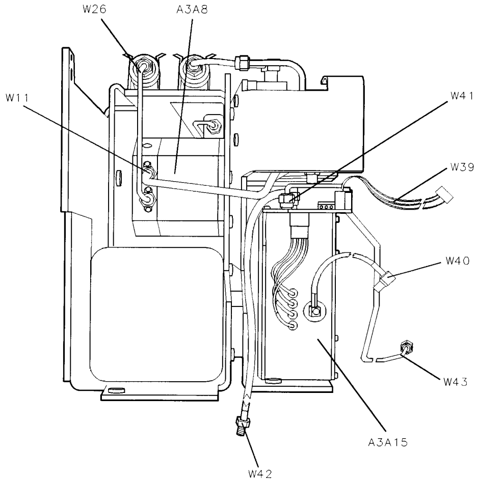
Figure 11-32. A3 Front-End Assembly, Rear View with A3A5 Removed HP 8595E and HP 8596E (Options 009 and 010)
