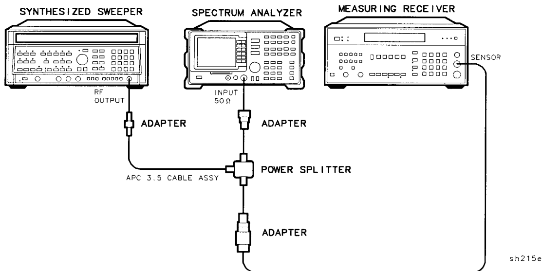
Figure 2-30. Frequency Response Setup
