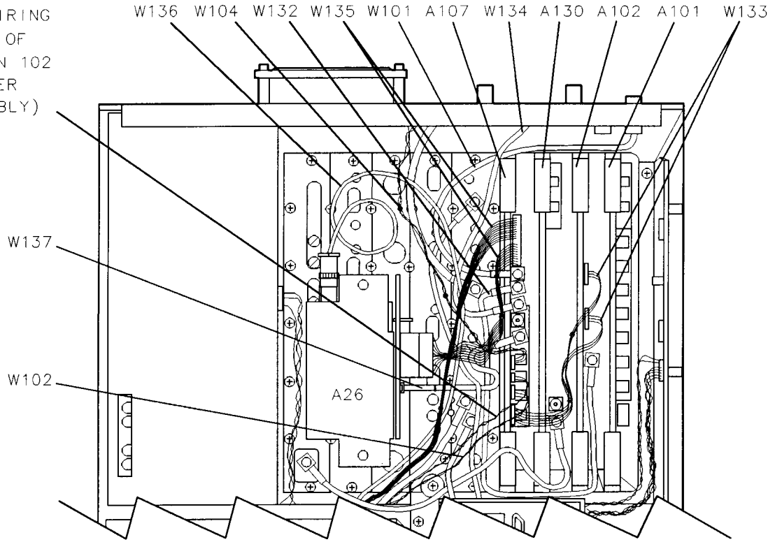
Figure 11-8. Card-Cage (Option 107) HP 8591C and HP 8590 E-Series
