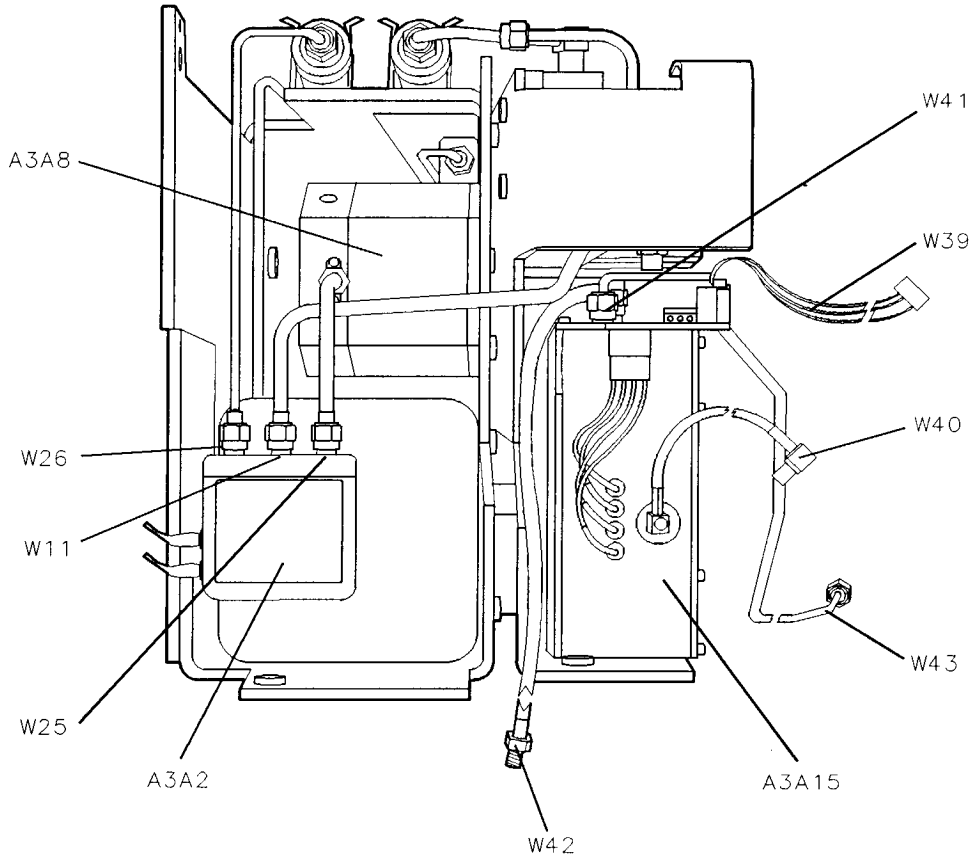
Figure 11-30. A3 Front-End Assembly, Rear View with A3A5 Removed HP 8593E (Options 009 and 010)
