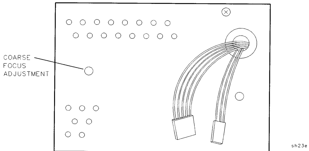
Figure 2-2. Coarse Focus Adjustment Location (rear view of display assembly)
