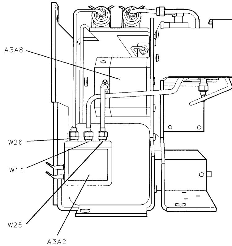
Figure 11-24. A3 Front-End Assembly, Rear View with A3A5 Removed HP 8592L and HP 8593E (Options 009 and 010)
