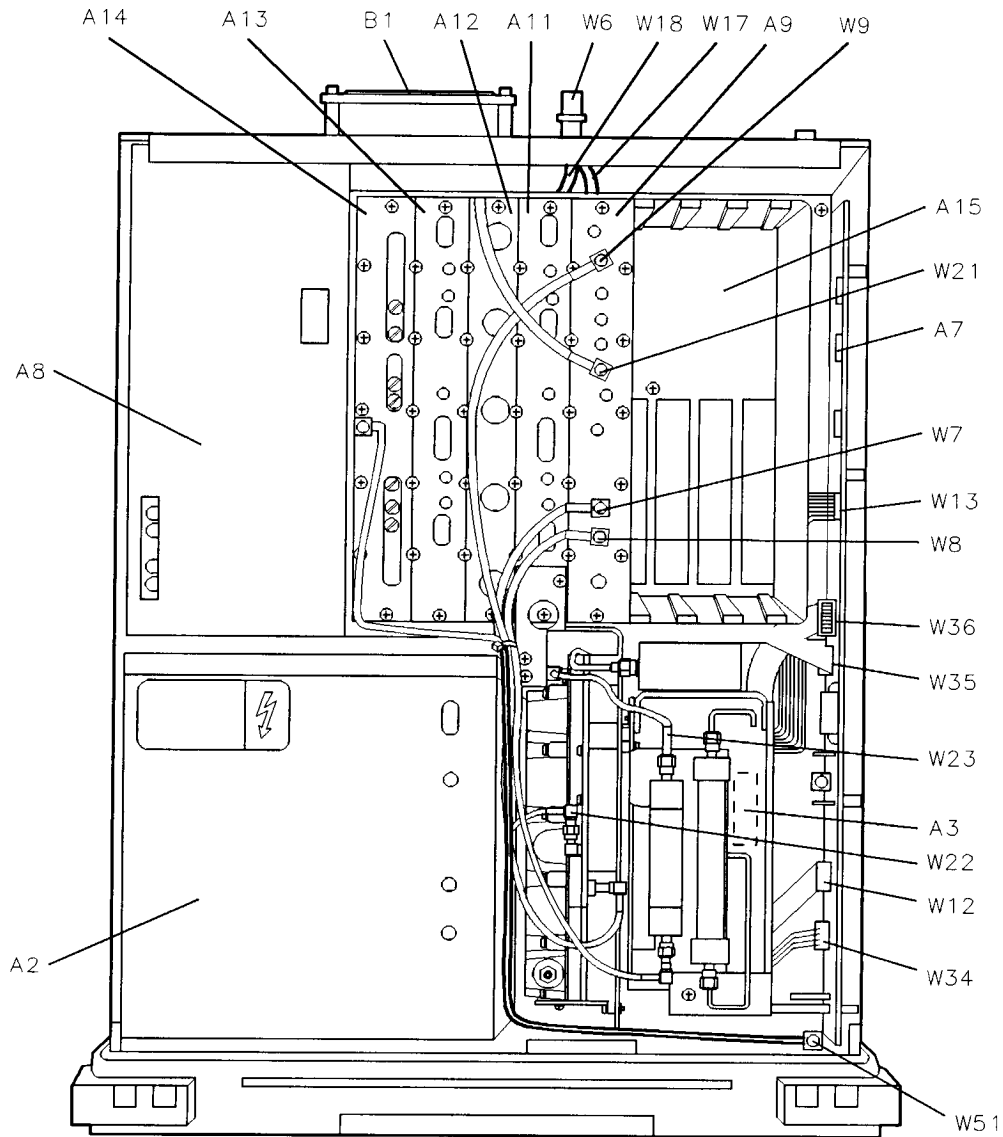
Figure 11-3. Instrument Top View HP 8592L, HP 8593E, HP 8594E, HP 8594L, HP 8594Q, HP 8595E, and HP 8596E
