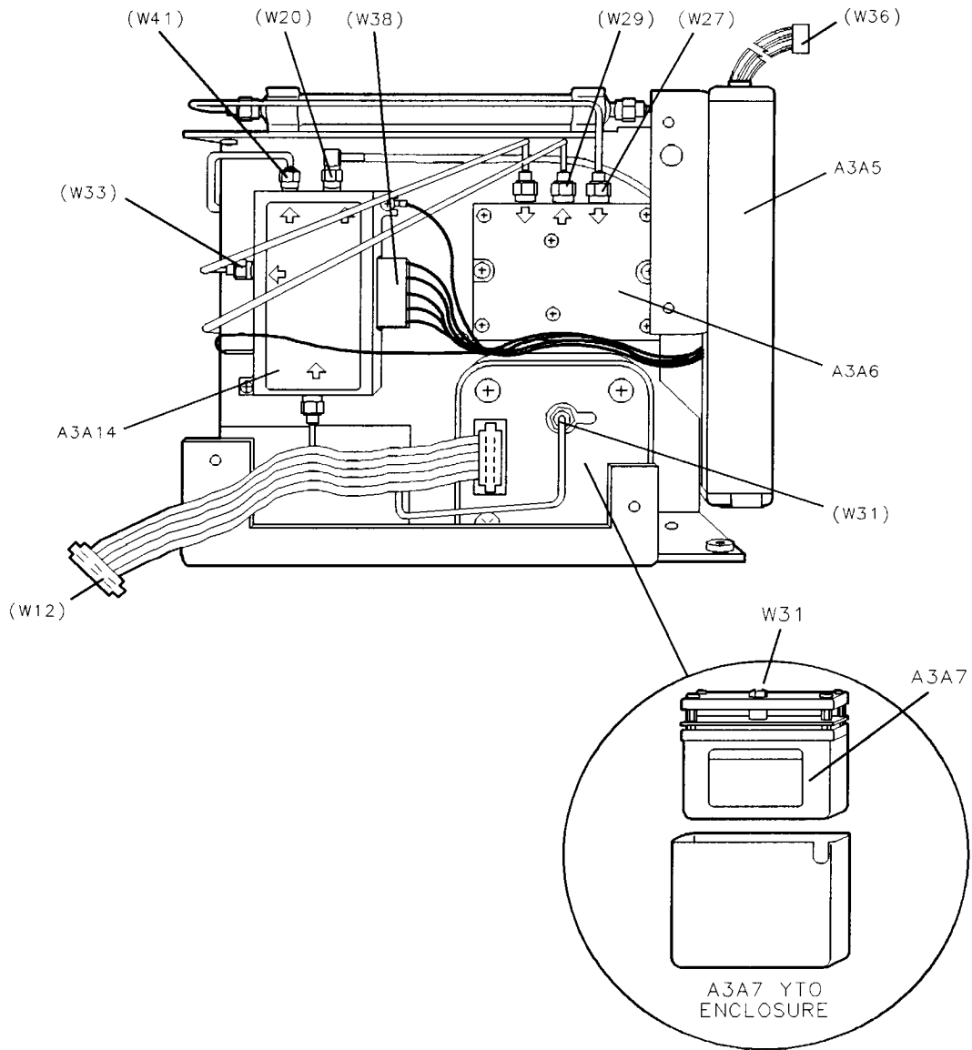
Figure 11-28. A3 Front-End Assembly, Right-Side View HP 8594E (Options 009 and 010)
