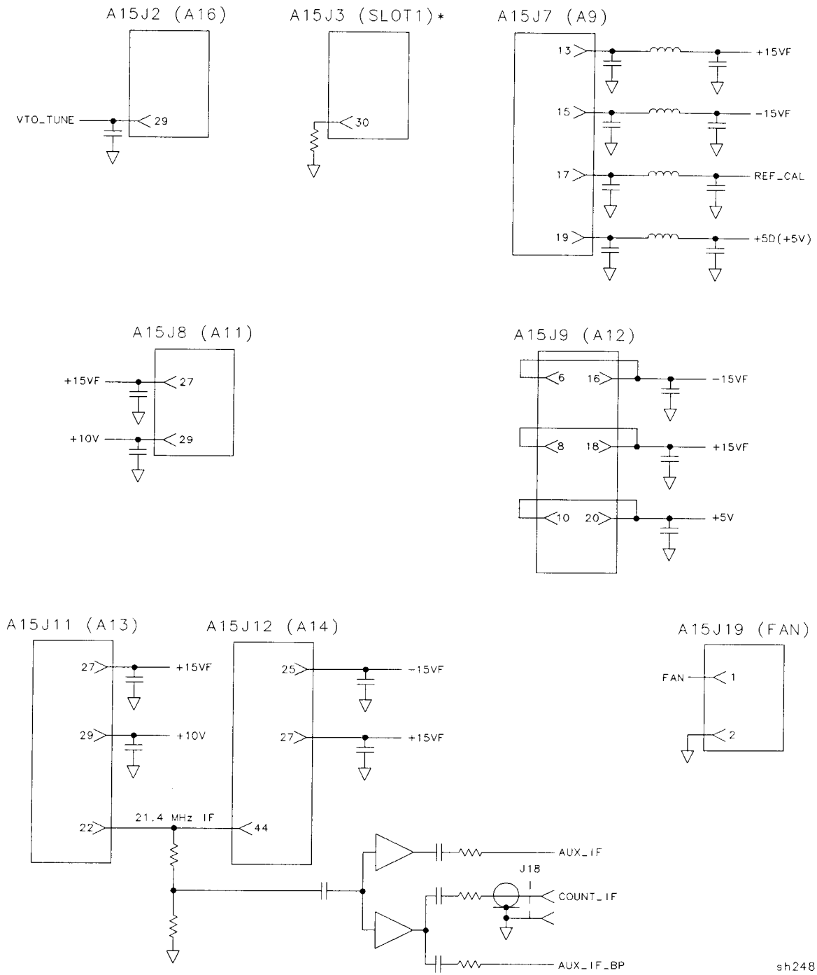
Figure 5-2. A15 Connectors with Additional Associated Circuitry (1 of 2)
