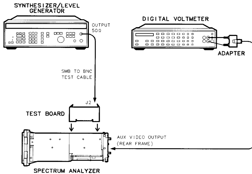
Figure 2-11. Log and Linear Amplifier Adjustment Setup
