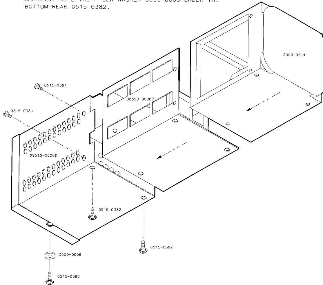
Figure 7-3. CRT Assembly
