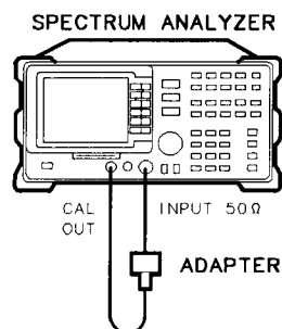
Figure 2-13. CAL FREQ Adjustment Routine Setup
