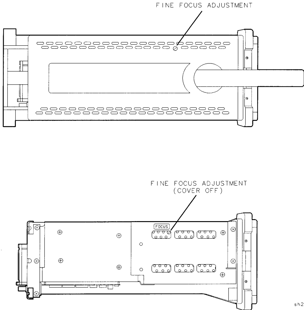
Figure 2-1. Fine Focus Adjustment Location
