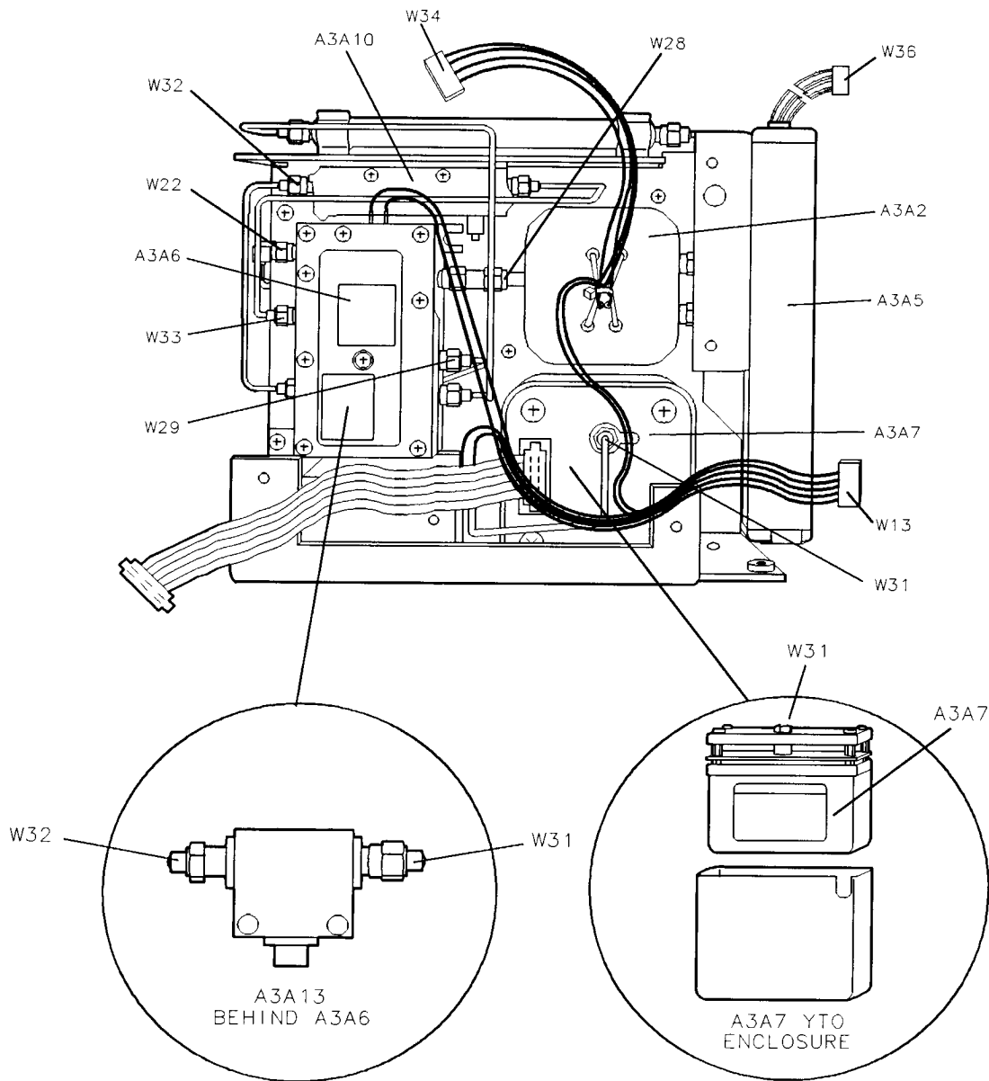
Figure 11-23. A3 Front-End Assembly, Right-Side View HP 8595E and HP 8596E
