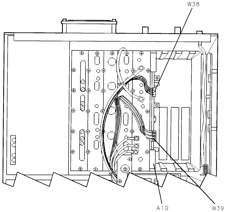
Figure 11-6. Card-Cage (Options 009, 010) HP 8593E, HP 8594E, HP 8594Q, HP 8595E, and HP 8596E
