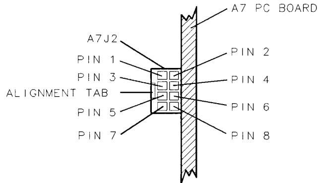
Figure 6a-1. A7J2 Pin-Out
