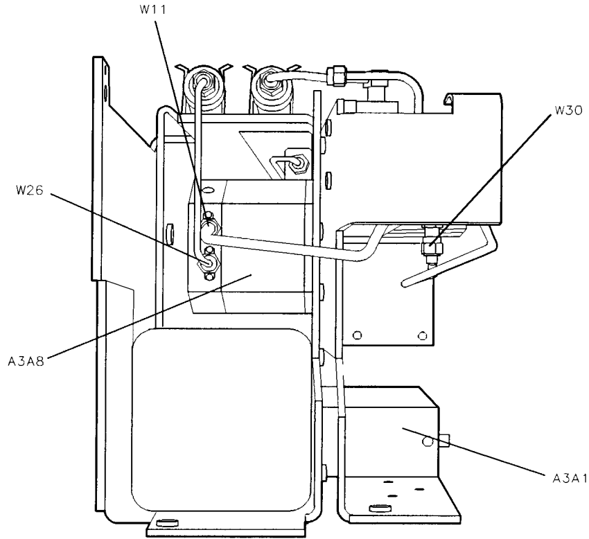
Figure 11-26. A3 Front-End Assembly, Rear View with A3A5 Removed HP 8595E and HP 8596E (Options 009 and 010)
