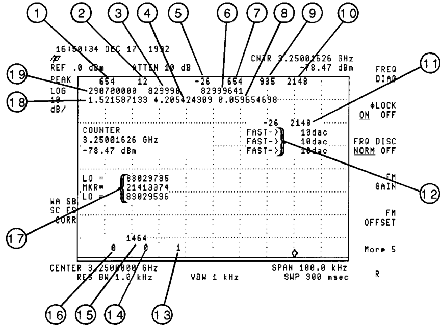
Figure 13-9. LO Frequency Diagnostic Data Display
